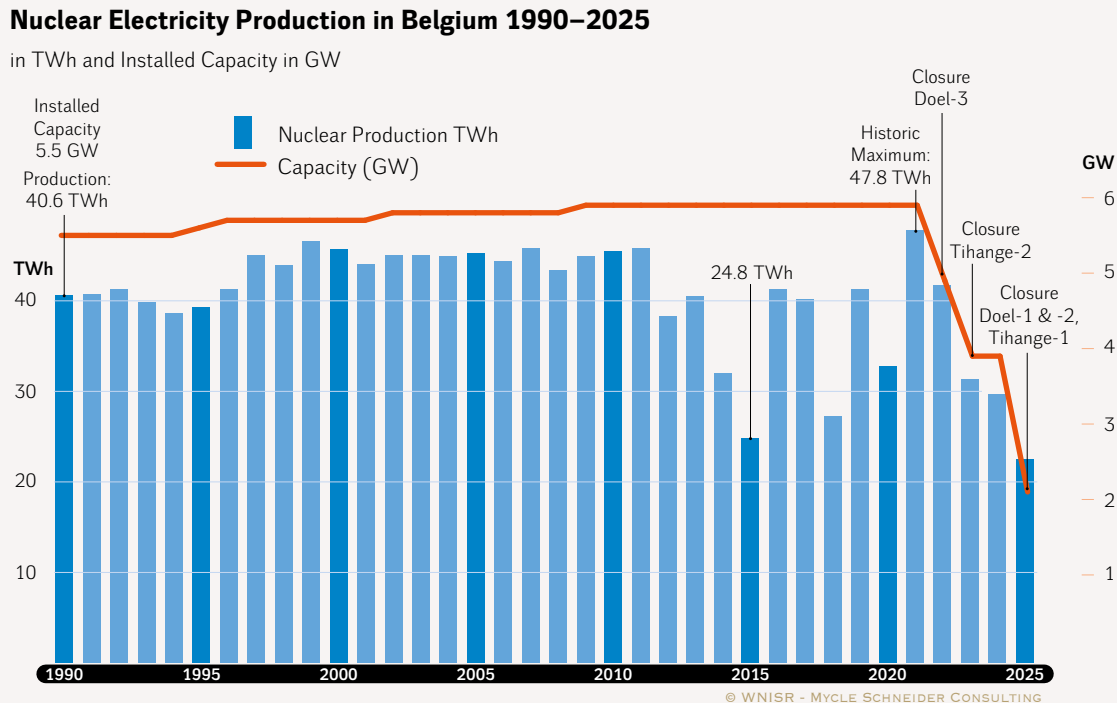
Figure 84 · Nuclear Power Generation in Belgium vs. Installed Nuclear Capacity
