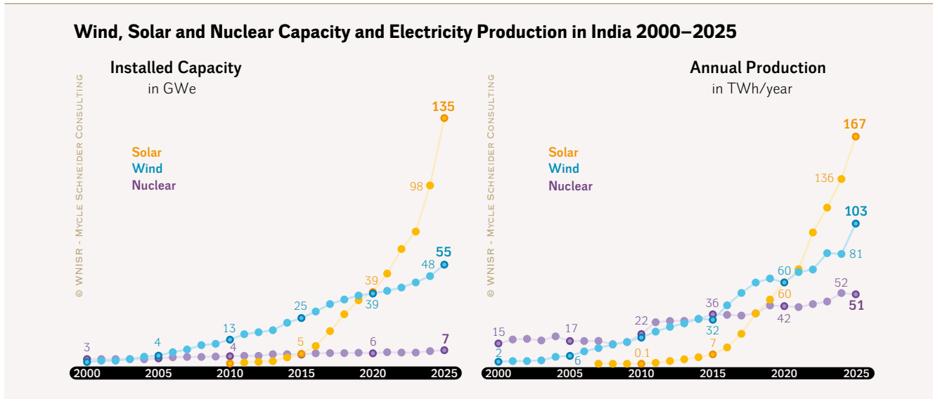
Figure 75 · Wind, Solar, and Nuclear Installed Capacity and Electricity Production in India
