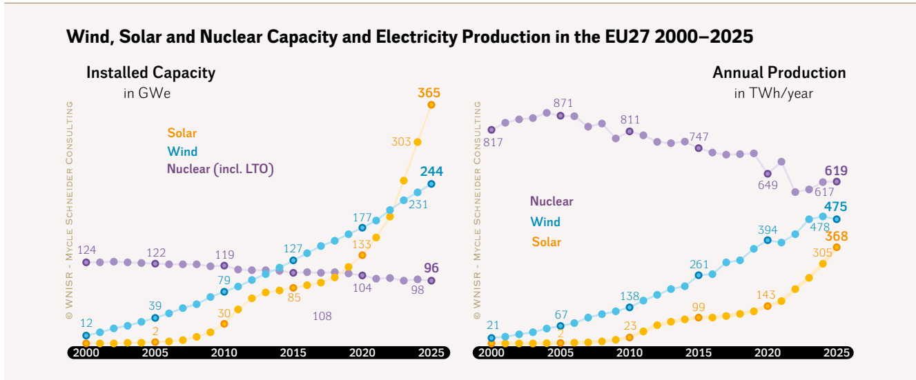
Figure 73 · Wind, Solar, and Nuclear Capacity and Electricity Production in the EU27
