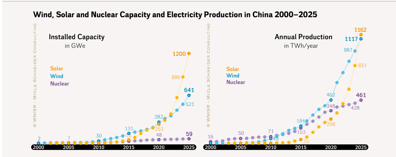
Figure 70 · Wind, Solar, and Nuclear Installed Capacity and Electricity Production in China
