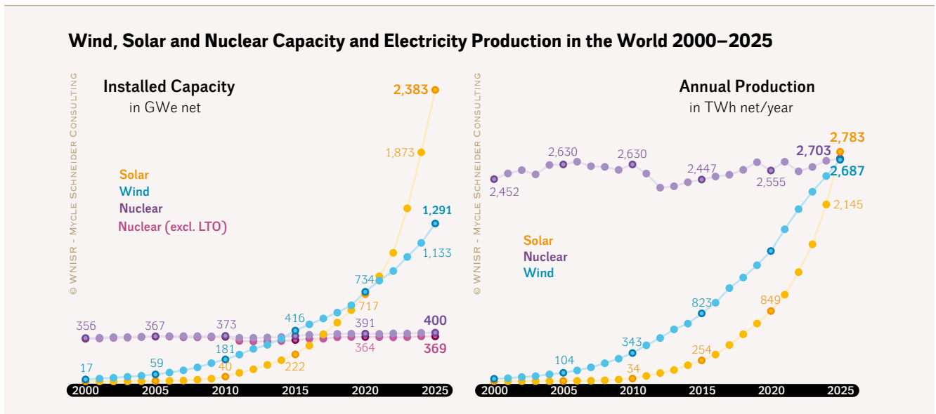
Figure 64 · Global Wind, Solar, and Nuclear Installed Capacity and Electricity Production
