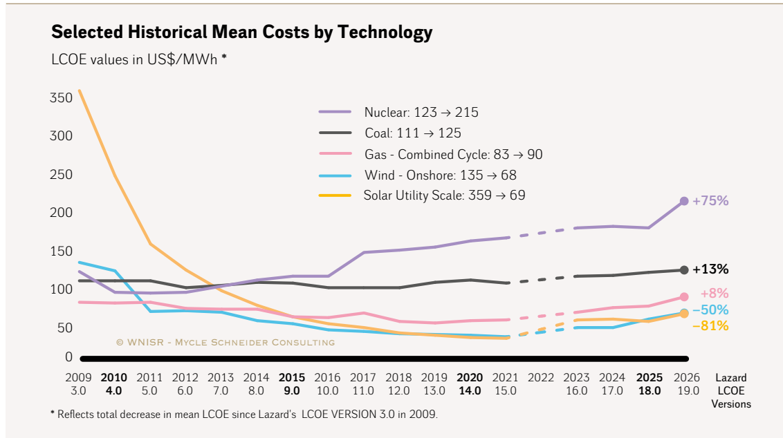
Figure 62 - The Declining Costs of Renewables vs. Traditional Power Sources
