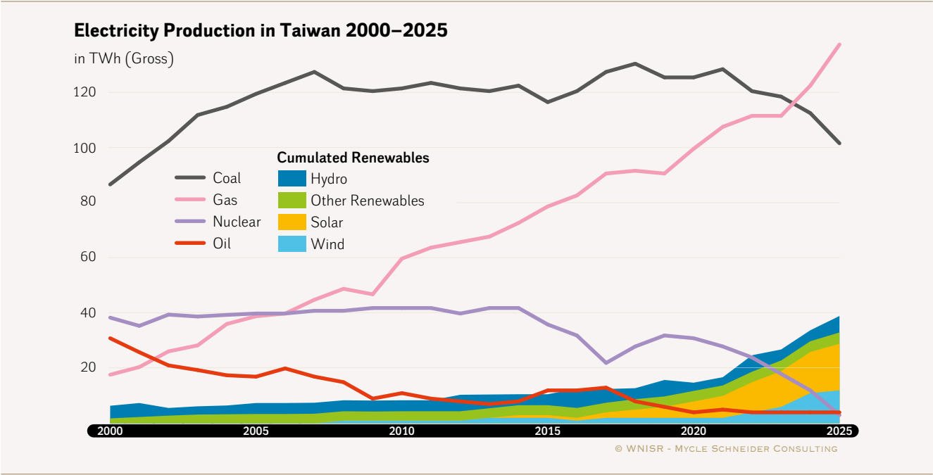
Figure 43 - Electricity Production in Taiwan, 2000–2025
