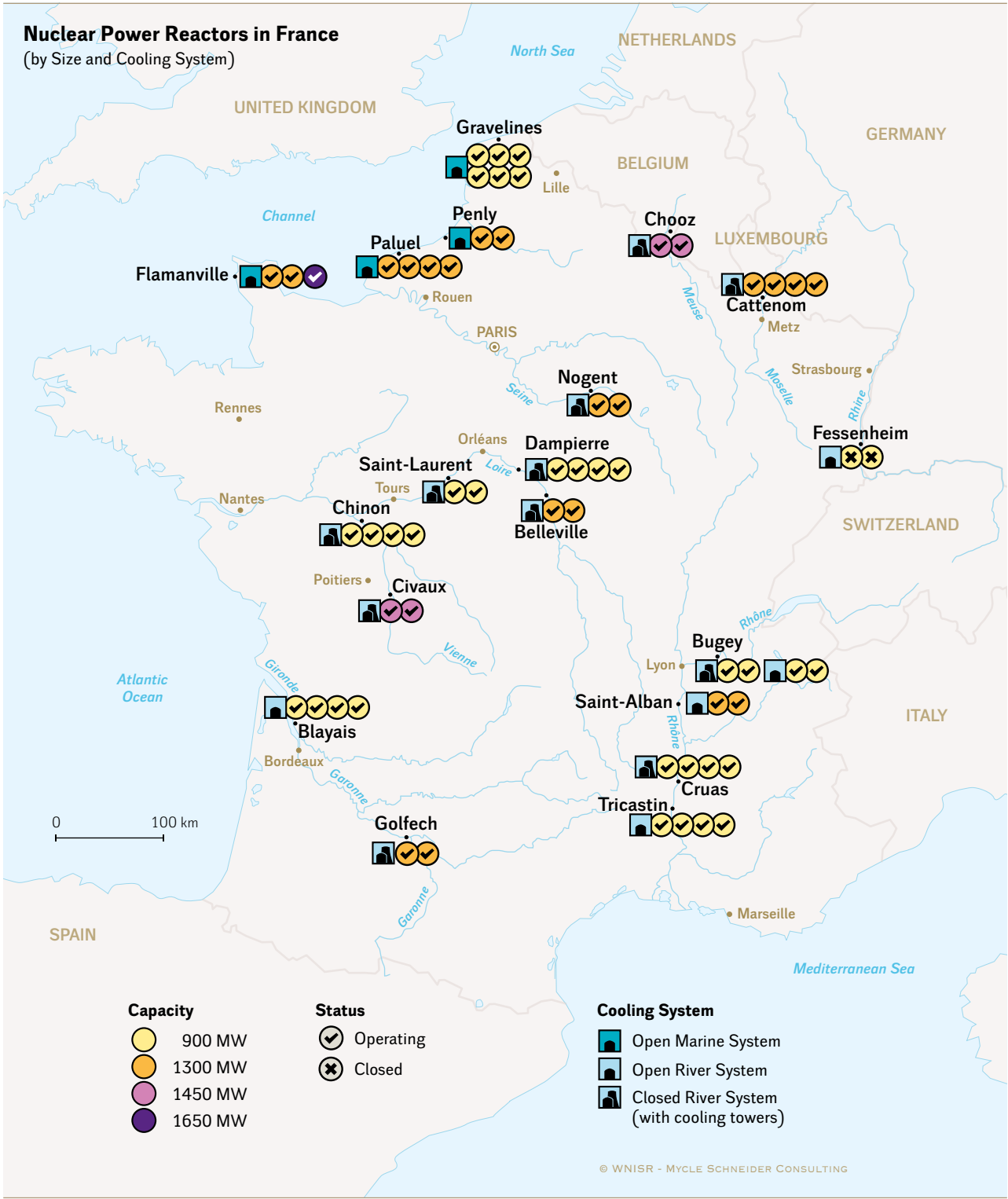
Figure 32 · Nuclear Power Reactors in France (by Size and Cooling System)
