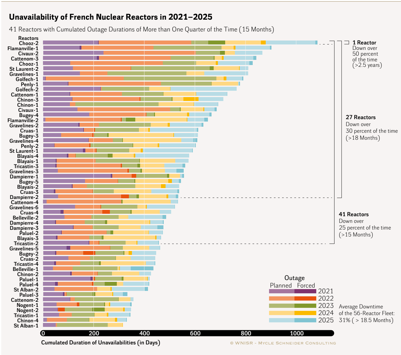
Figure 29 · Unavailabilities of French Nuclear Reactors, 2021–2025
