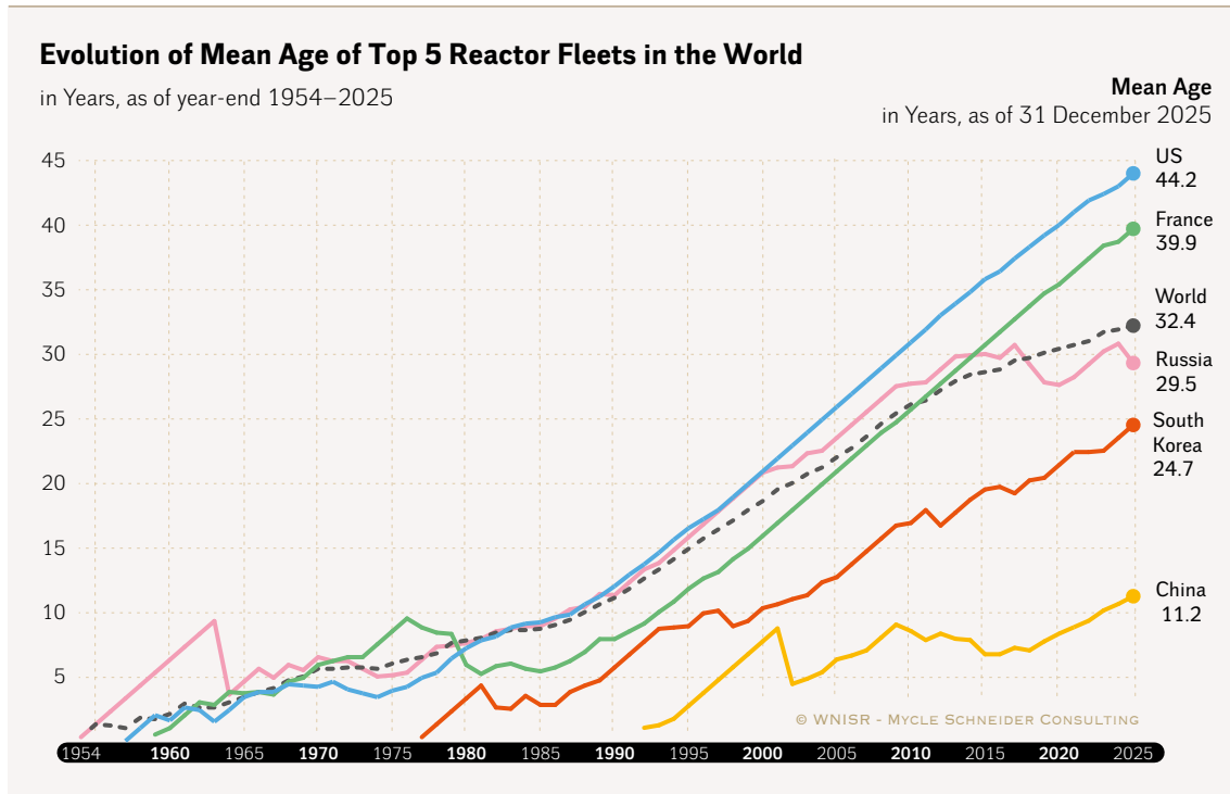
Figure 16 · Reactor-Fleet Age of Top 5 Nuclear Generators
