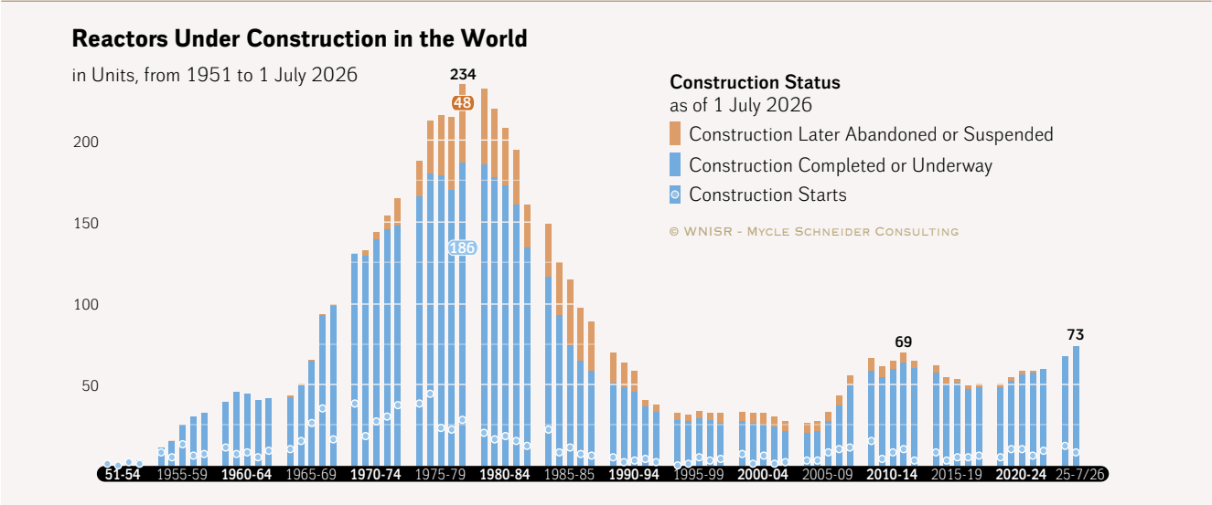
Figure 7 · Nuclear Reactors “Under Construction” in the World
