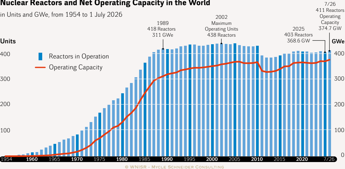
Figure 6 · World Nuclear Reactor Fleet, 1954–mid-2026
