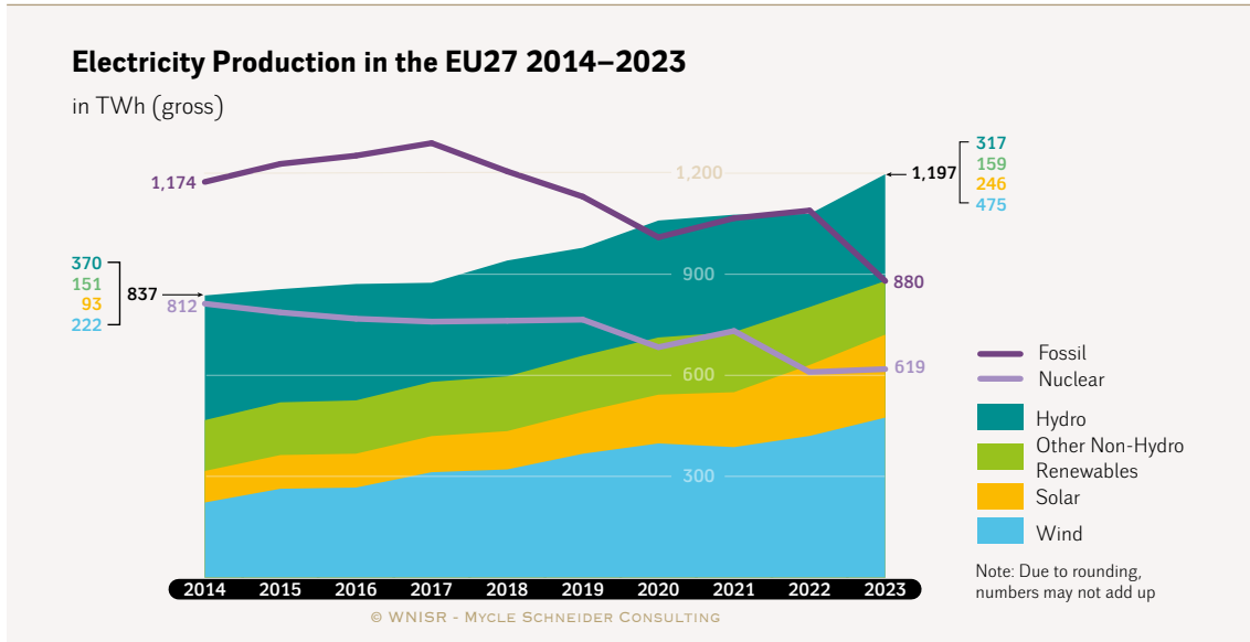
Figure 65 • Electricity Generation in the EU27 by Fuel, 2013–2023
