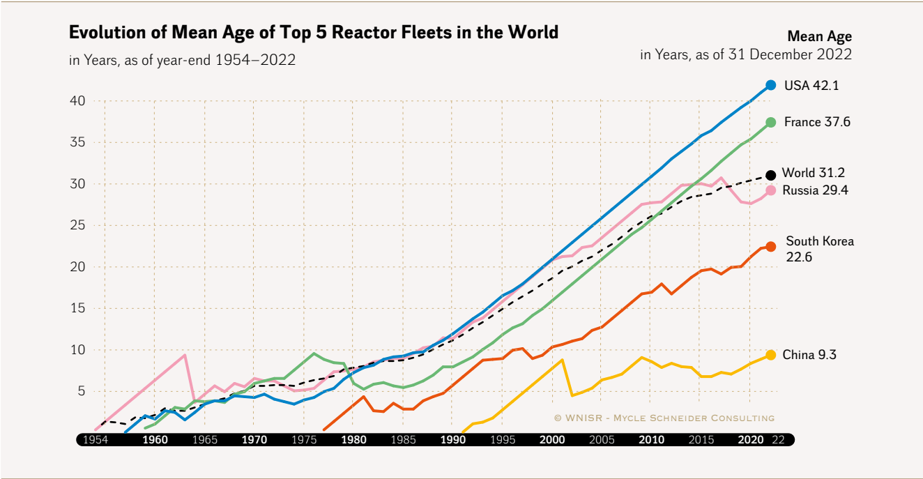
Figure 19 • Reactor-Fleet Age of Top 5 Nuclear Generators
