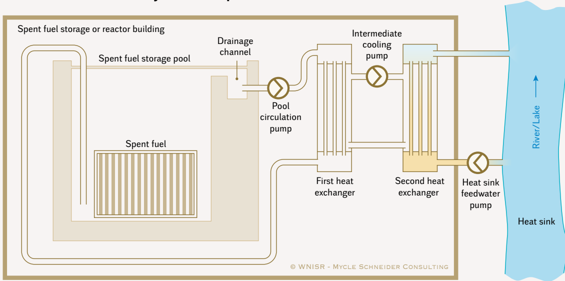
Figure 48 · Spent Fuel Pool Residual-Heat Removal System
